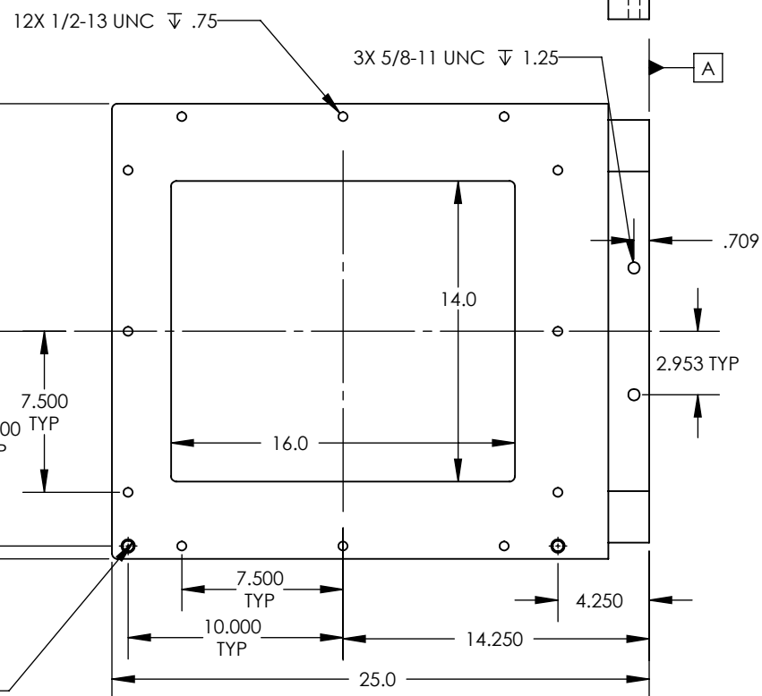
2-SIDED WINDOW ANGLE PLATE
